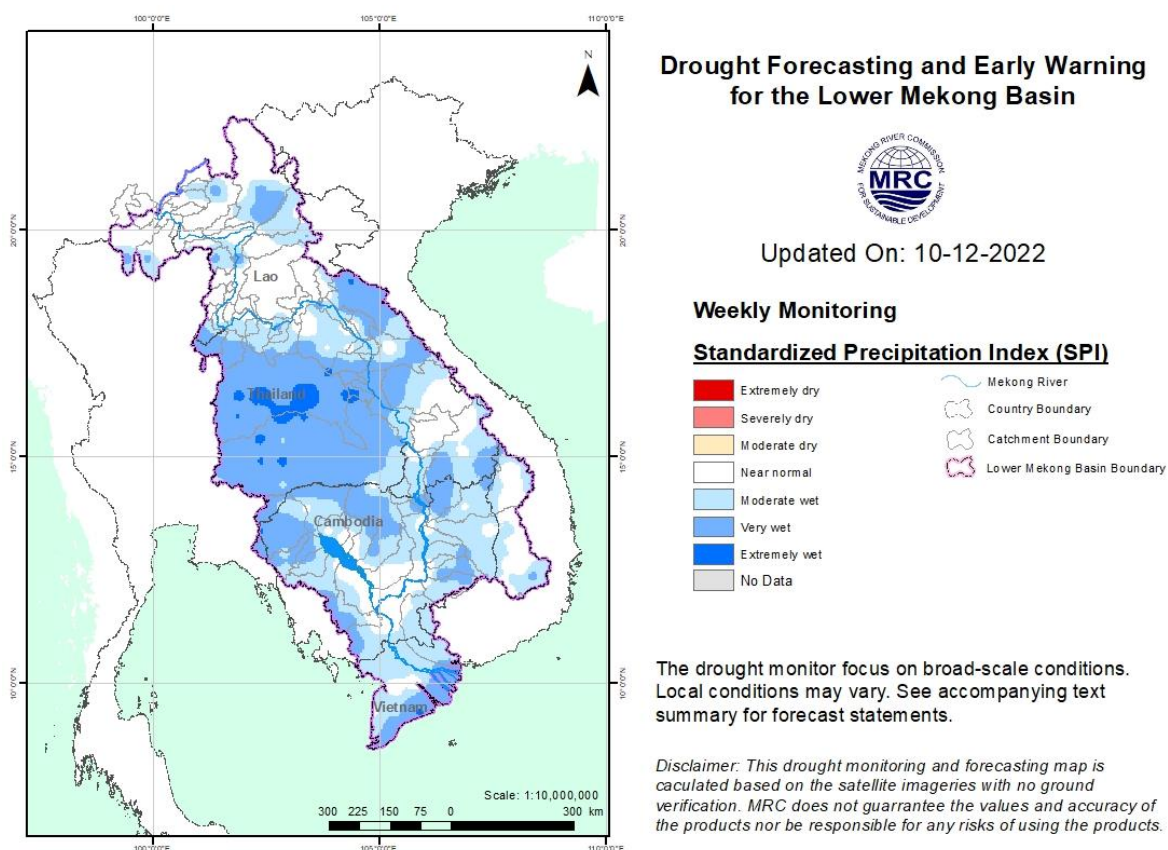
Figure 14: Weekly standardised precipitation index from December 4 to 10.
