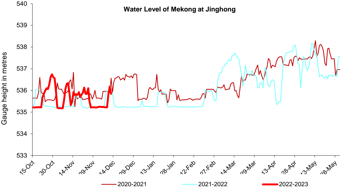
Figure 7. Water level at the Jinghong hydrological station during to 12 Dec 2022.
