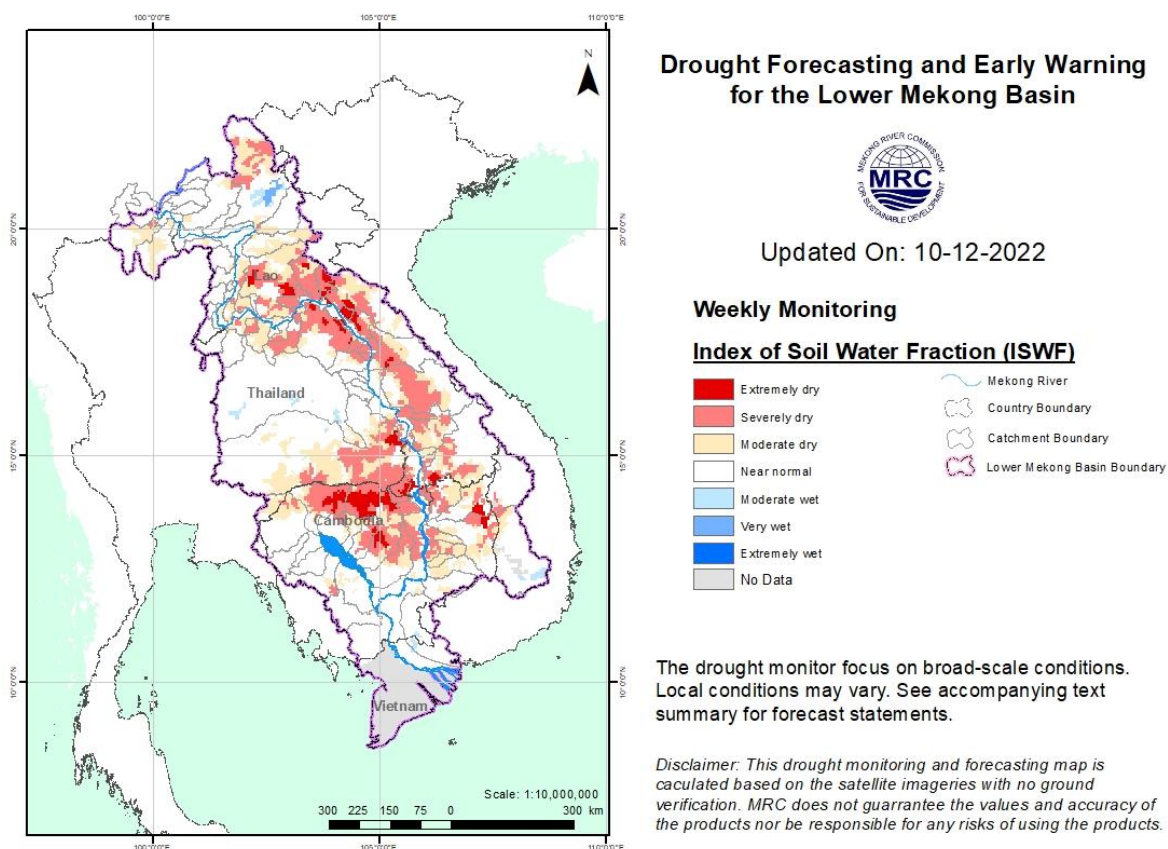
Figure 15: Weekly Index of Soil Water Fraction from December 4 to 10.
