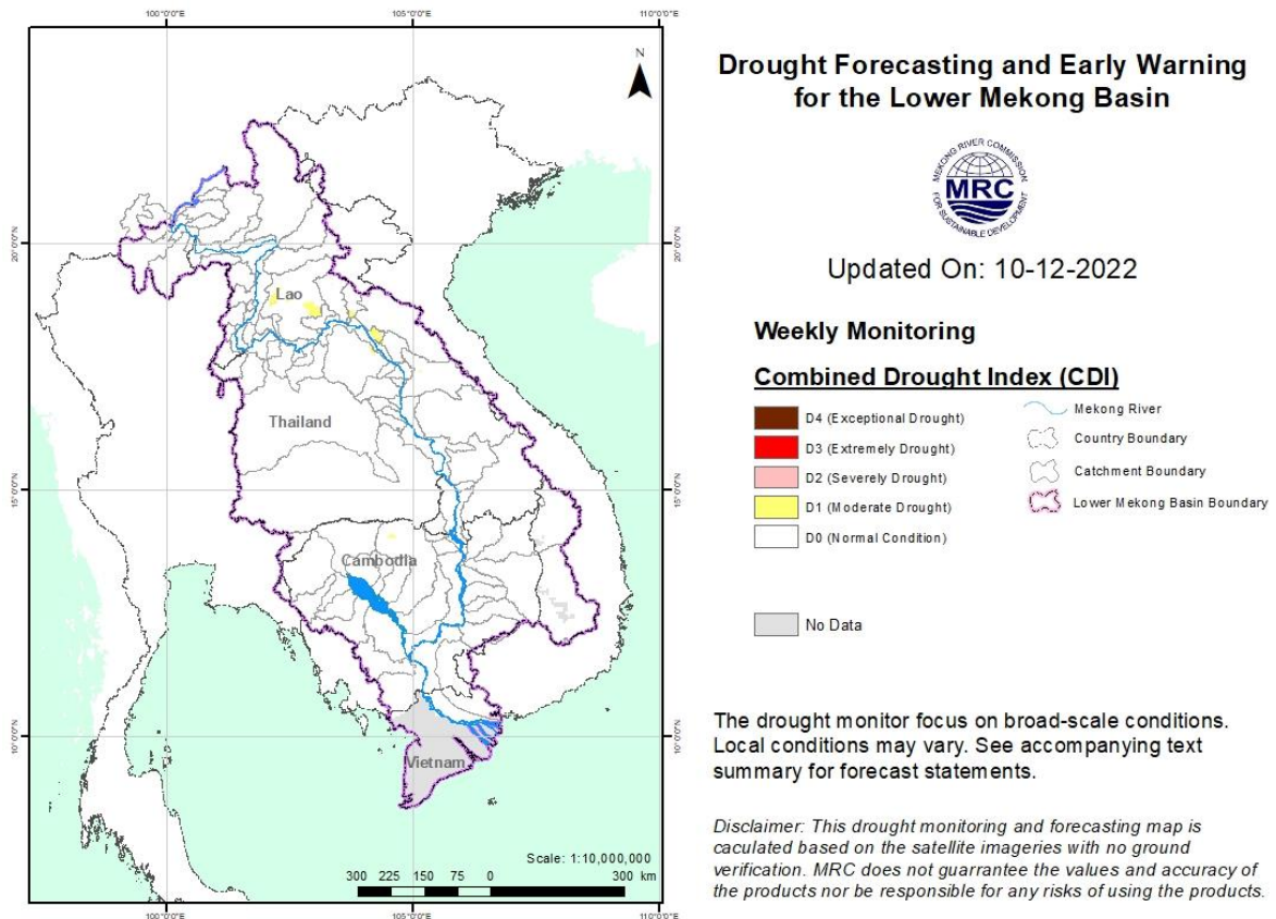
Figure 16: Weekly Combined Drought Index during November 27-December 3.
