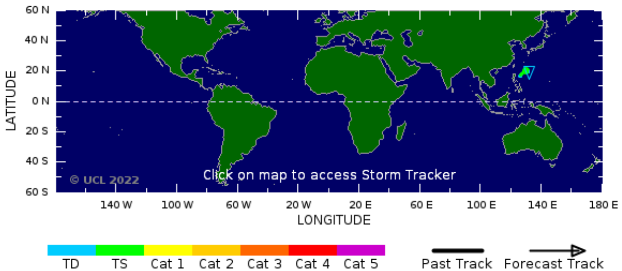
Figure 3: No tropical storm risk observed on 12 December 2022.
